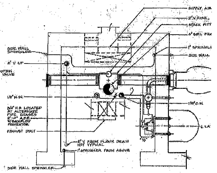
3 CHASE PIPING LOWER LEVEL TYPICAL P. 6 SCALE 1/2" = 1'-0"
