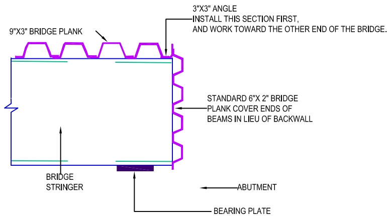
TYPICAL END TREATMENT
