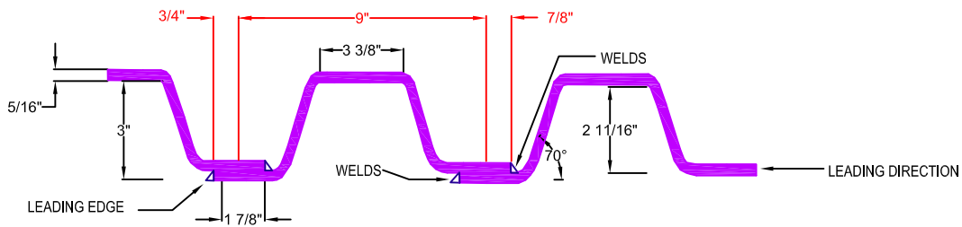
CROSS SECTION - BRIDGE PLANK
