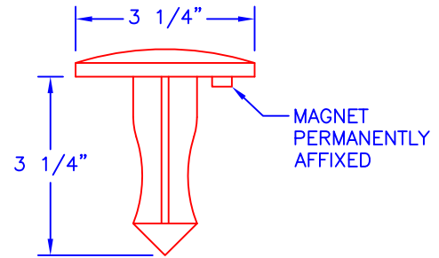
BRASS CAP
