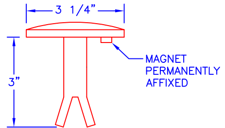
ALUMINUM CAP
