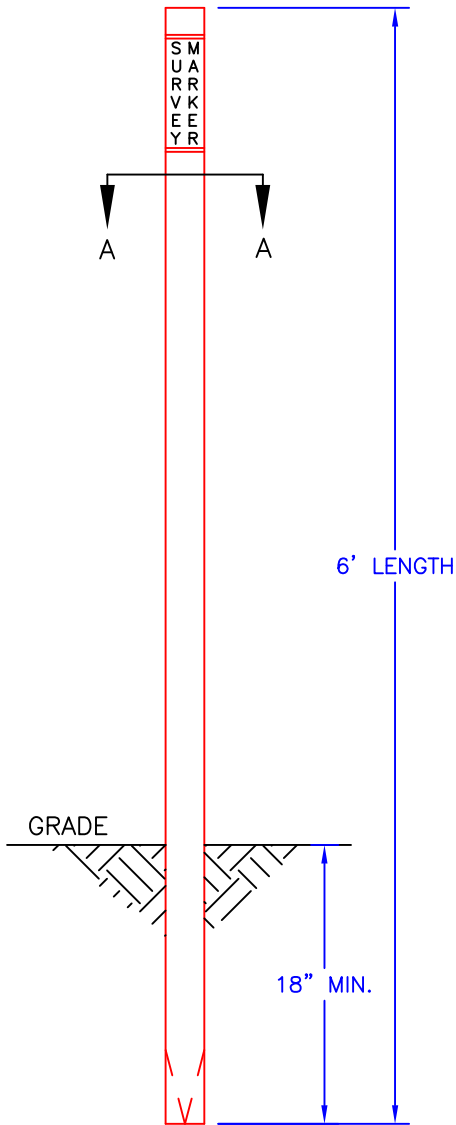
WITNESS POST
